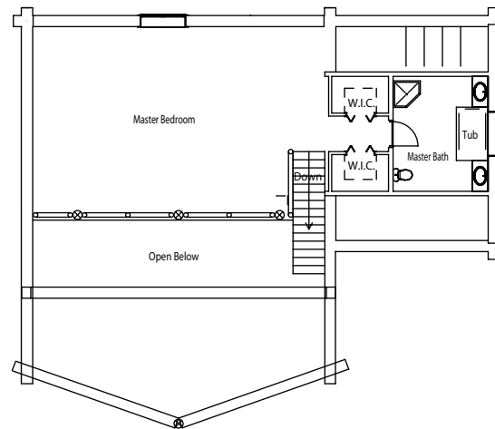
Loft Floor Plan 937 sqft
