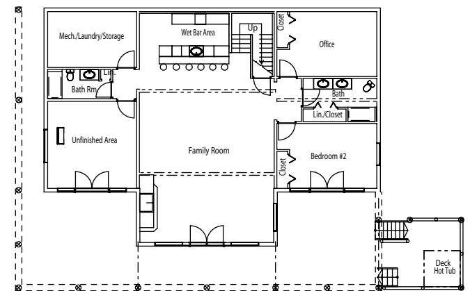
Suggested Lower Level Floor Plan
